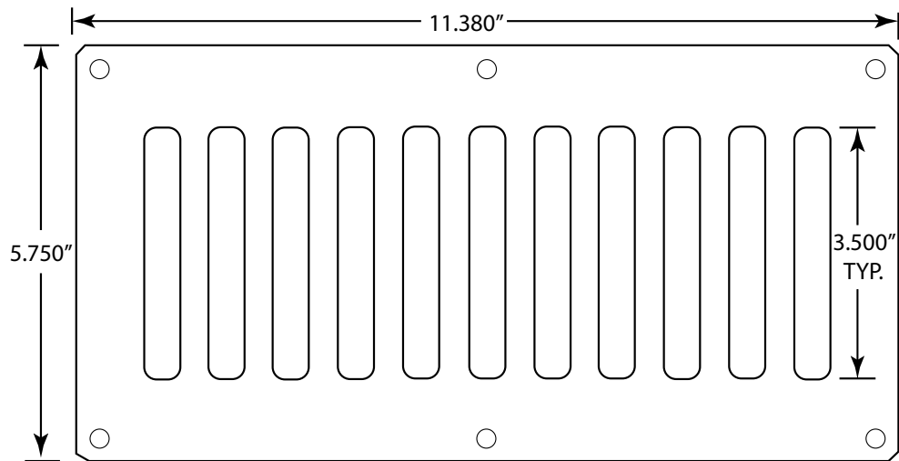
Fig. 1 Vent dimensions.
