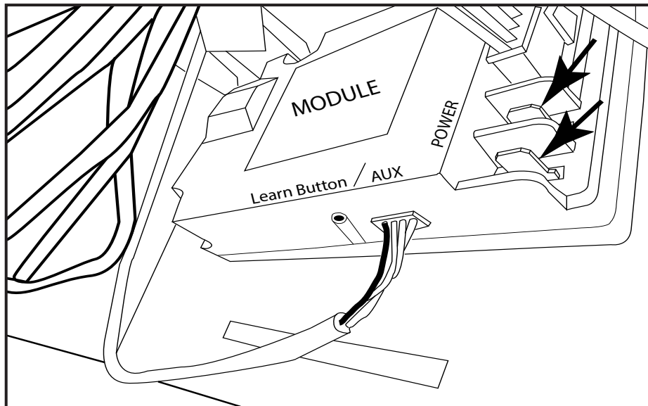
Fig. 2 Shows location of control module's two ¼" terminals (labeled POWER) to attach adapter.
