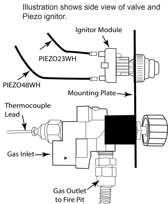
Fig. 5 TMSI typical installation.
