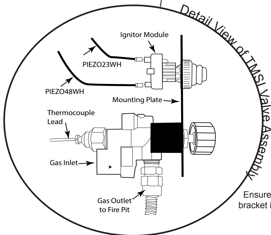
Fig. 8 Typical installation.
