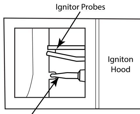
Fig. 6 Proper alignment of probes and thermocouple.
