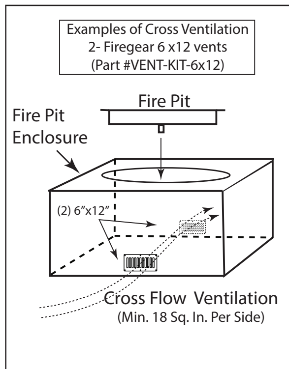
Fig 3. Cross Ventilation Example
