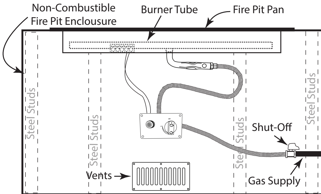
Fig. 6 Typical installation.
