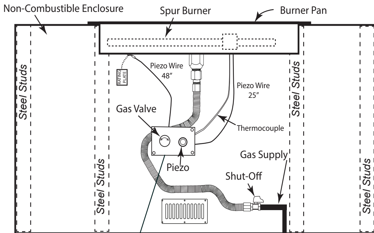
Fig. 6 Typical installation.
