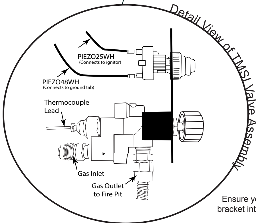
Fig. 7 Typical installation.
