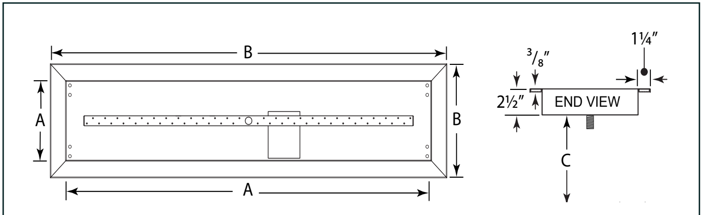
Fig. 2 T-style burner pan specifications.
