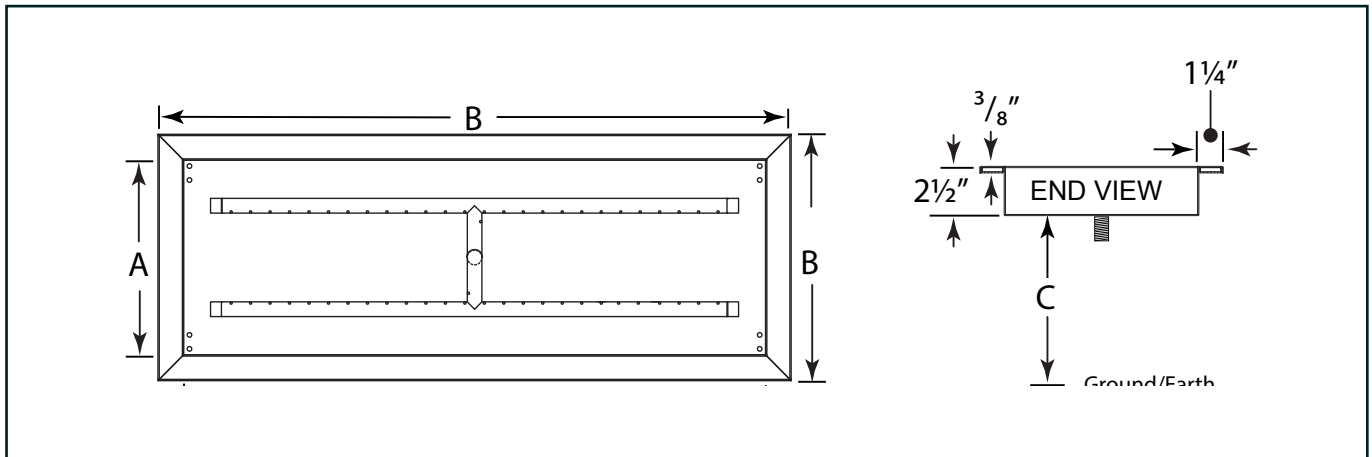
Fig. 1 H-style burner pan specifications.
