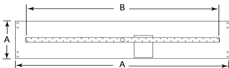
Fig. 1 T-style burner pan specifications.
