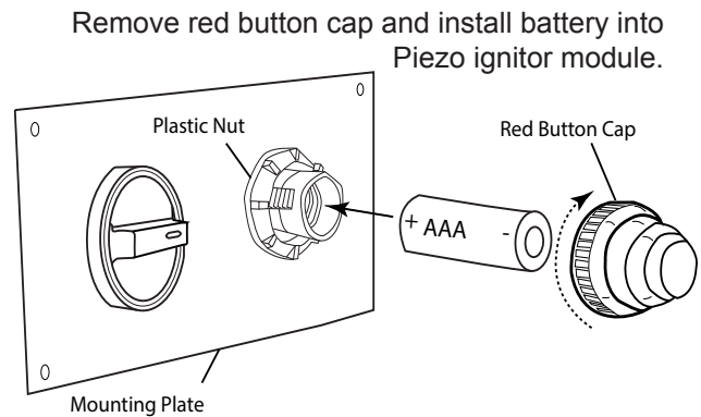
Fig. 9 Installing battery into Piezo.
