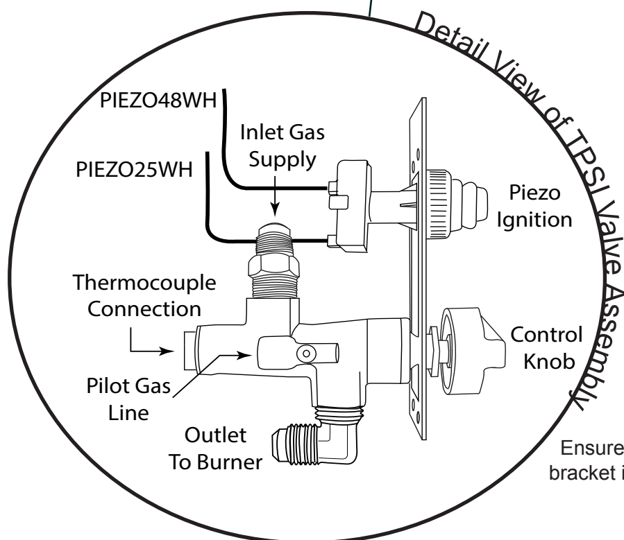
Fig. 11 Typical installation.
