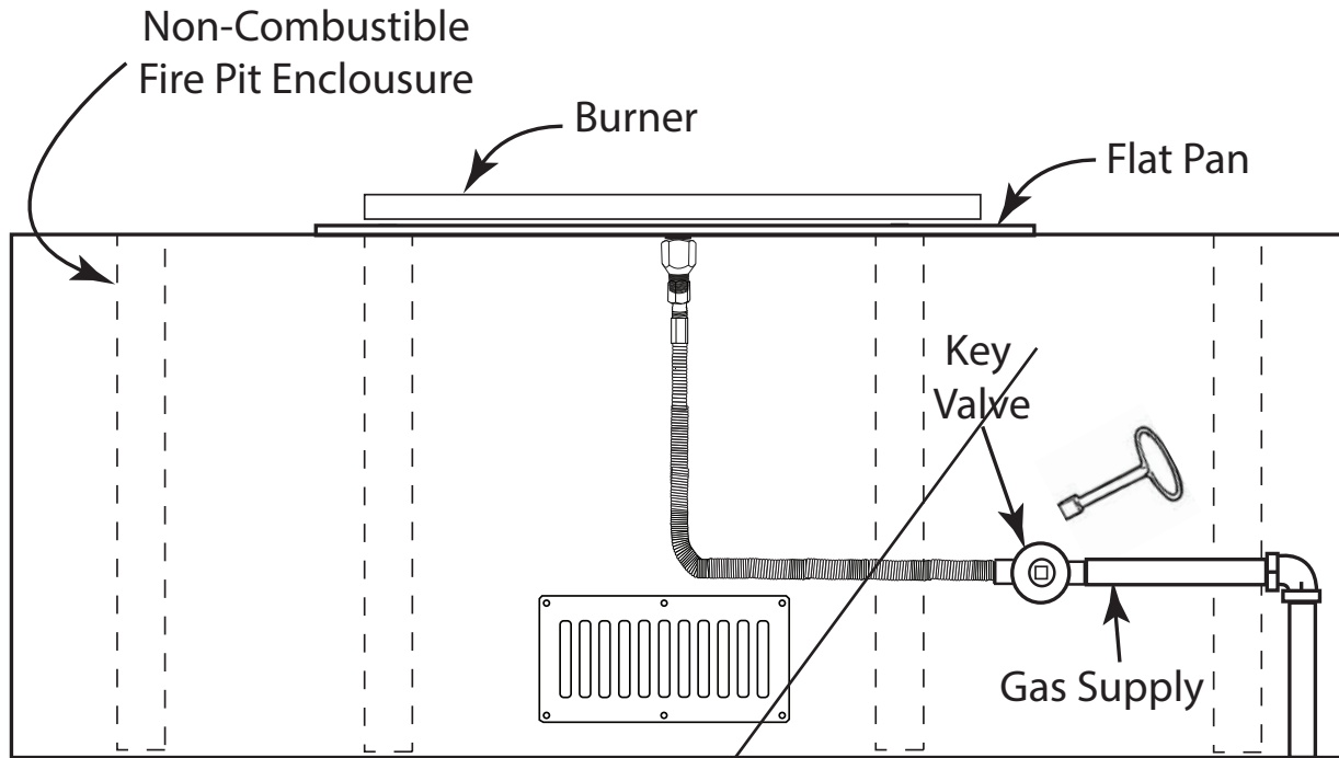
Fig. 5 Typical Installation
