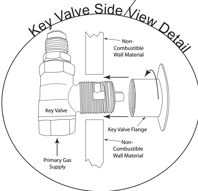
Fig. 7 Typical installation.
