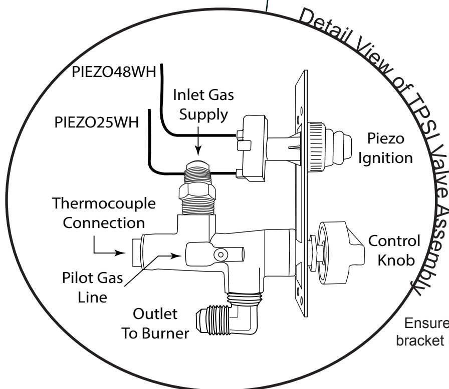
Fig. 12 Typical installation.
