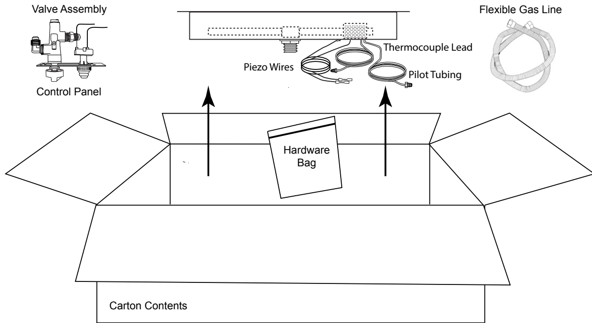
Fig. 5 Removing contents from carton.
