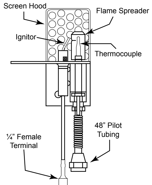
Fig. 10 Show TPSI pilot assembly identification.
