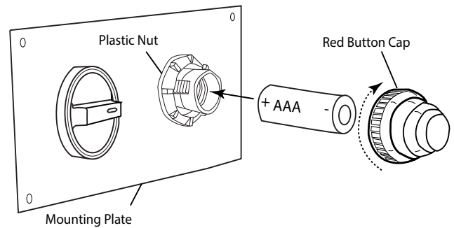
Fig. 9 Installing battery into Piezo.
