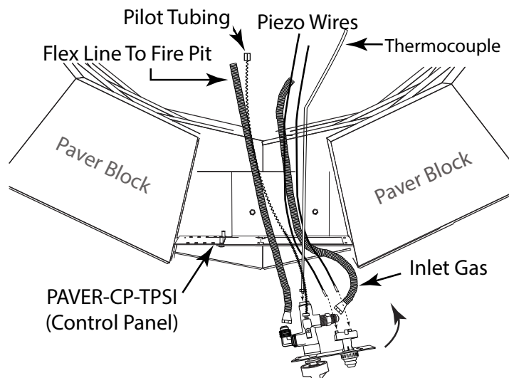
Fig. 7 Installing control panel into PAVER-CP-TPSI mounting plate.
