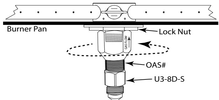
Fig. 6 Installing OAS assembly to spur burner.
