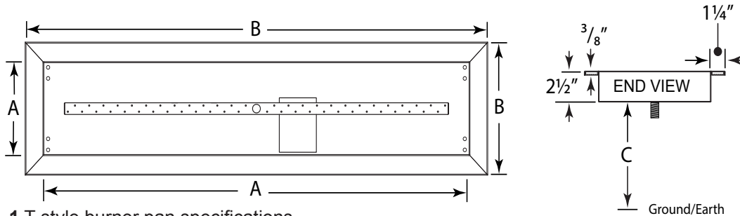
Fig. 1 T-style burner pan specifications.
