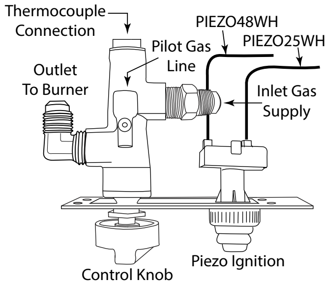
Fig. 8 TPSI control panel mounting plate.
