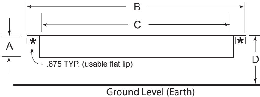
Fig 1. Fire pit dimensions; refer to Table 1.
