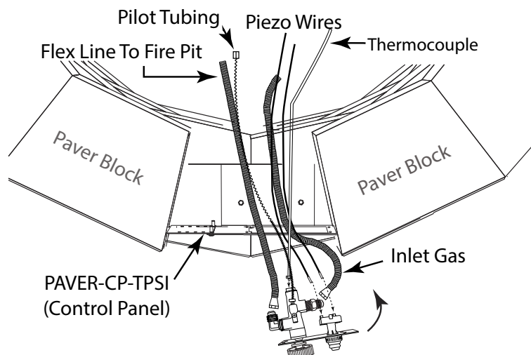
Fig. 6 Installing control panel into PAVER-CP-TPSI mounting plate.
