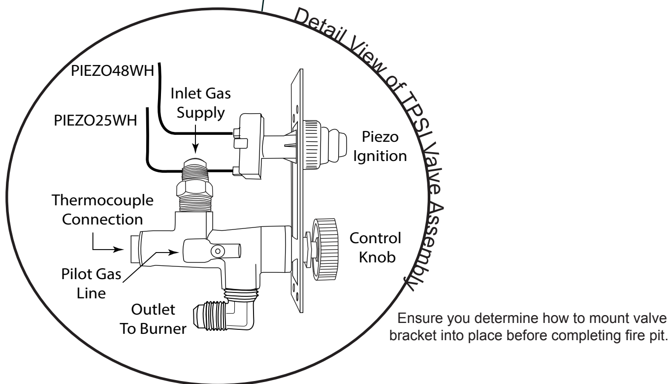
Fig. 11 Typical installation.
