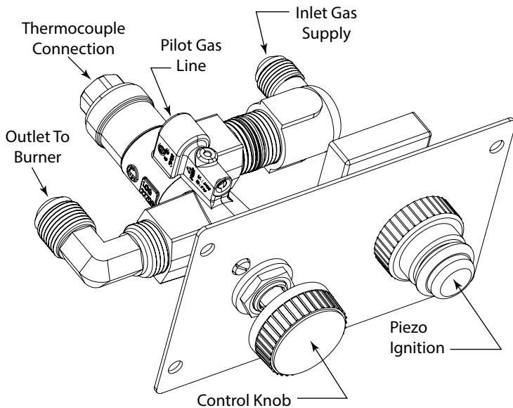
Fig. 7 TPSI control panel mounting plate.
