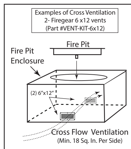
Fig 3. Cross Ventilation Example
