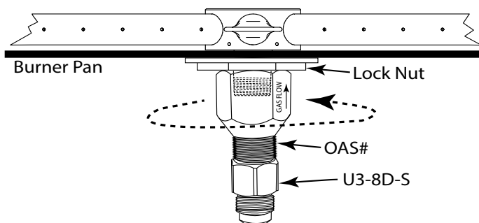
Fig. 5 Installing OAS assembly to spur burner.
