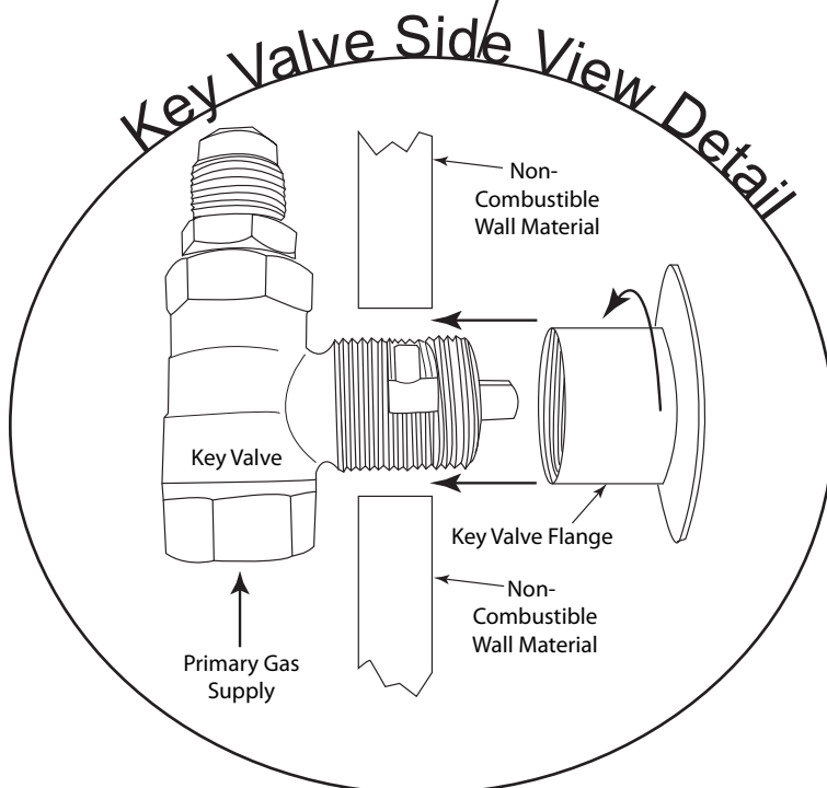
Fig. 5 Typical installation.
