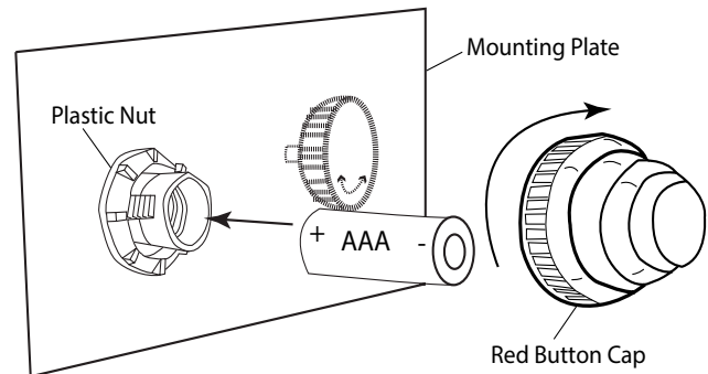
Fig. 9 Installing battery into Piezo.
