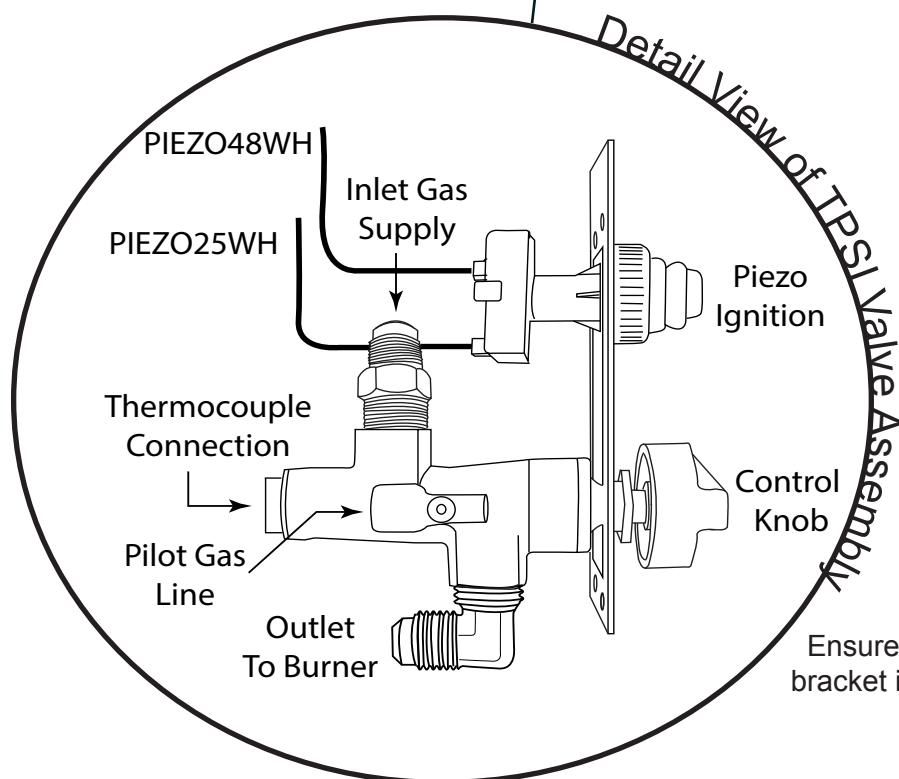
Fig. 12 Typical installation.
