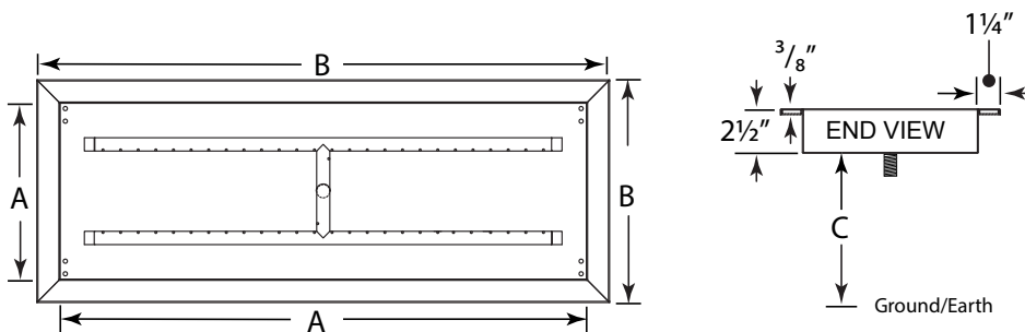
Fig. 1 H-style burner pan specifications.
