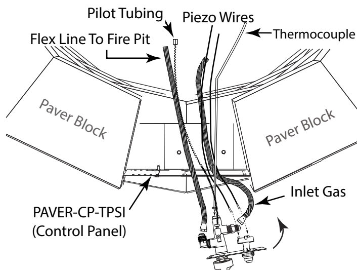
Fig. 7 Installing control panel into PAVER-CP-MT mounting plate.
