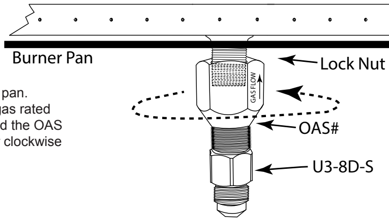
Fig. 5 Installing OAS (orifice) to burner tube.
