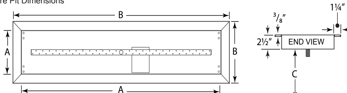
Fig. 3 T-style burner pan specifications.
