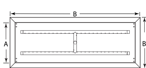
Fig. 1 H-style burner pan specifications.
