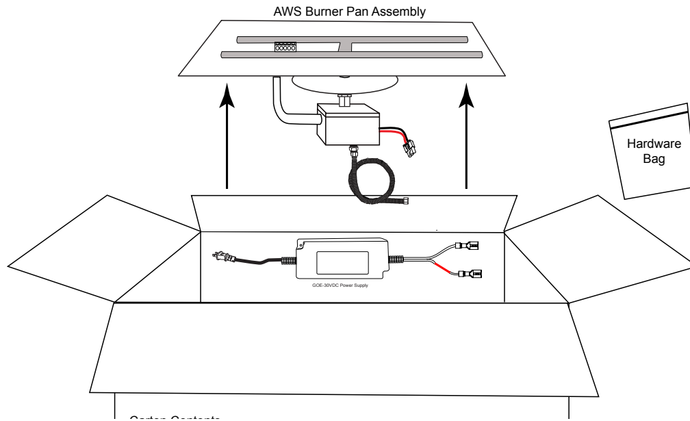
Fig. 8 Shows carton contents. Note: An H-burner was illustrated for this drawing.
