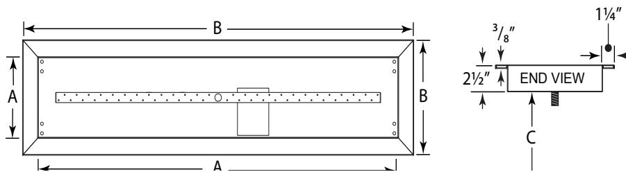
Fig. 3 T-style burner pan specifications.
