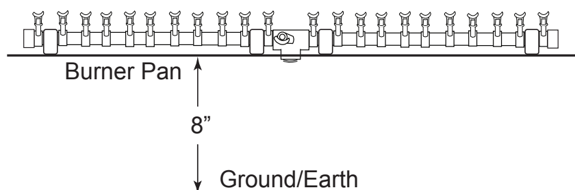
Fig. 1 T-style flat burner pan specifications.
