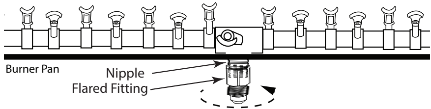
Fig. 5 Installing gas line to Pro Burner.
