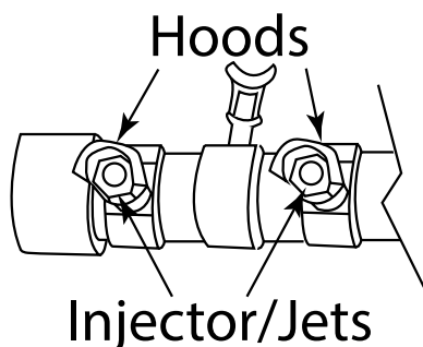
Fig. 10 Correct placement of injector hoods.
