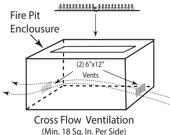
Fig. 3 Shows cross ventilation for a linear enclosure.
