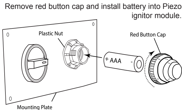
Fig. 8 Installing battery into Piezo.
