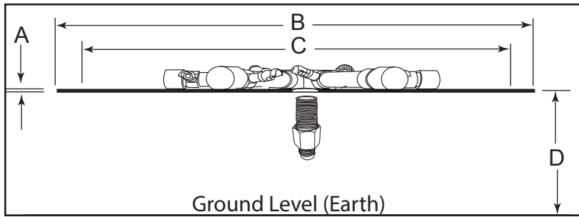
Fig. 1 Fire Pit Dimensions; refer to Table 1. (Dimensions applicable to round or square pans)
