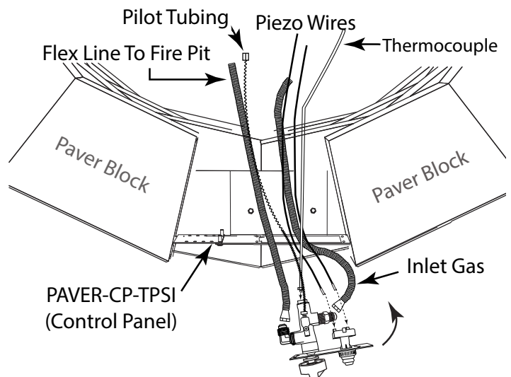
Fig. 5 Installing control panel into PAVER-CP-TPSI mounting plate.
