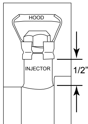
Fig. 12 Shows 1/2" spacing from bottom of injector.
