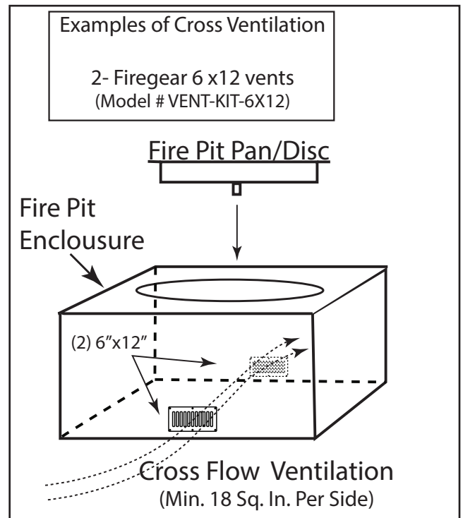
Fig. 6 Cross Ventilation Example
