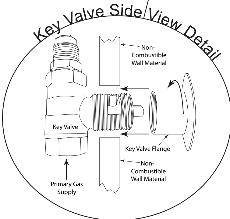
Fig. 7 Typical installation.
