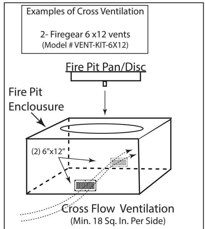
Fig. 5 Cross Ventilation Example
