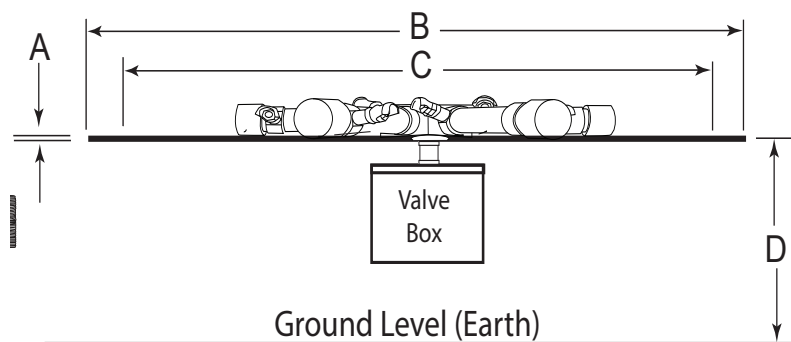
Fig. 1 Shows disc side view.
