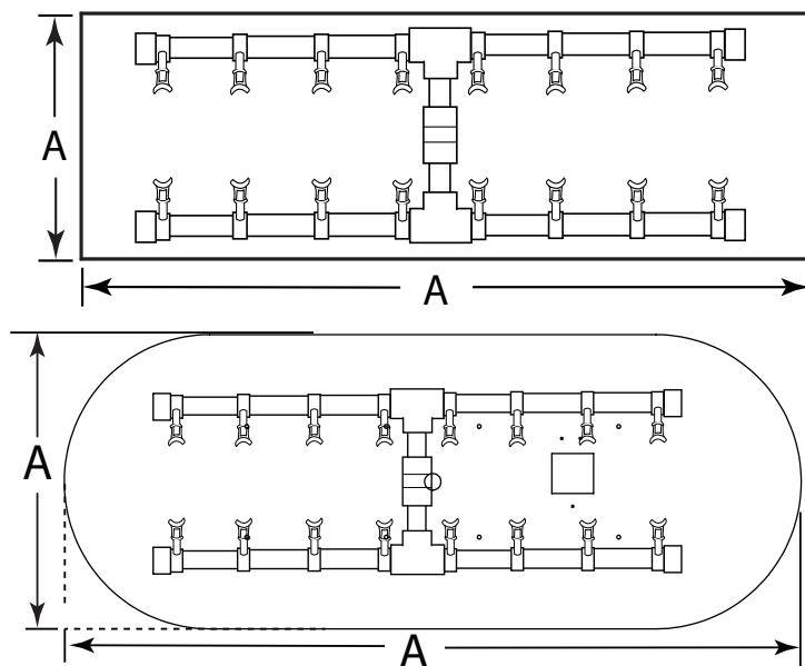
Fig. 1 H-style flat burner pan specifications.
