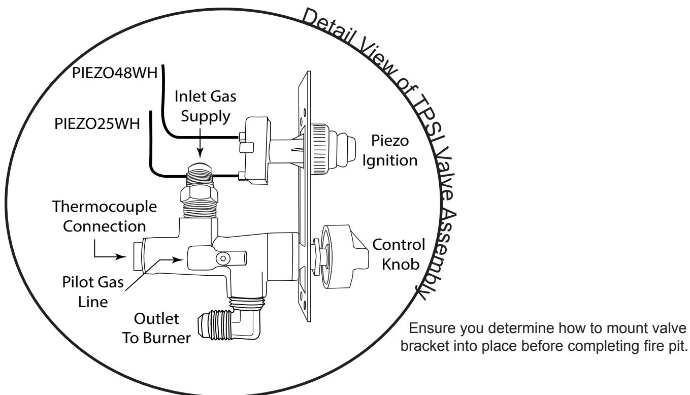
Fig. 12 Typical installation.
