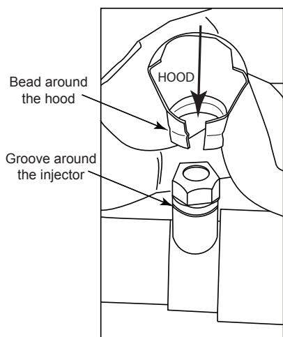
Fig. 10 Installing hood over top of injector.
