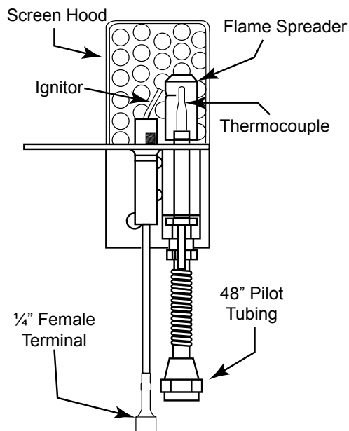
Fig. 8 Show TPSI pilot assembly identification.
