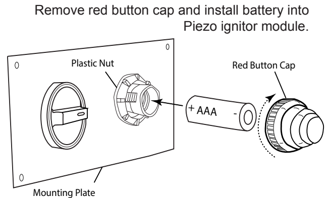
Fig. 7 Installing battery into Piezo.
