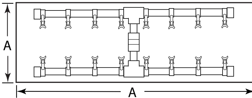
Fig. 1 H-style flat burner pan specifications.
