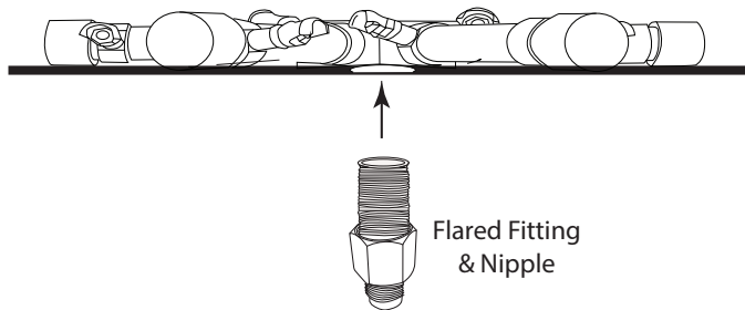
Fig. 4 Installing nipple into bottom of burner.
