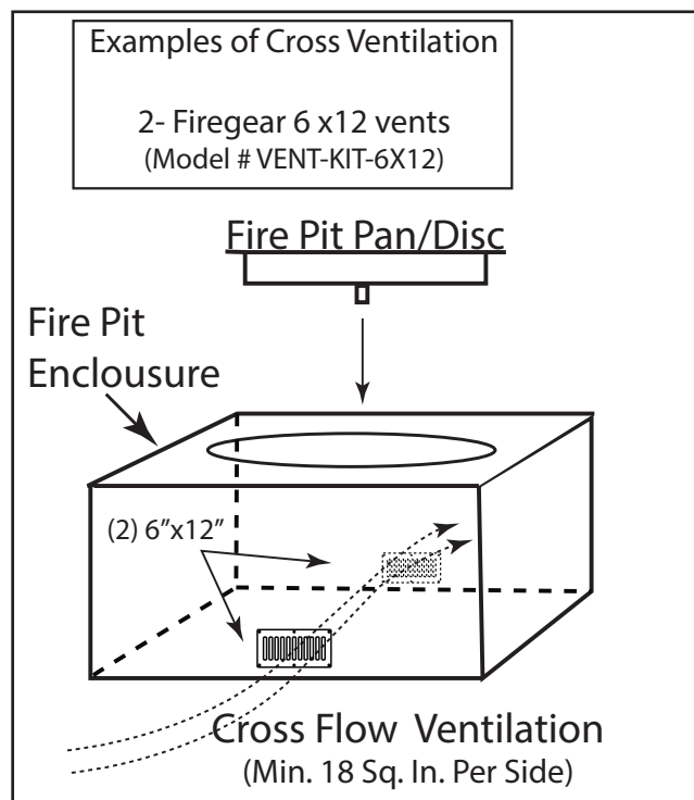
Fig. 5 Cross Ventilation Example
