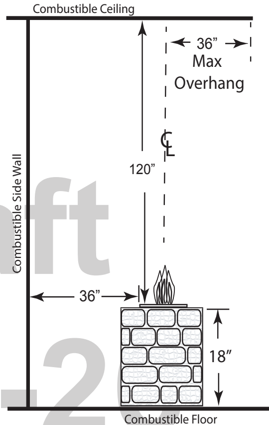
Fig. 2 Clearance to combustibles
