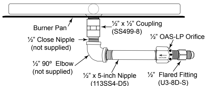
Fig. 12 Optional LP conversion illustration shows a 90° elbow and close nipple (not supplied).
